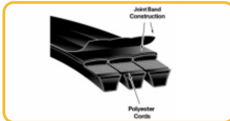
Banded V Belt as per ISO 5290 (RA/RB/RC, R5V/R8V, BB/CC, 2~8 Bands, up to 8890 mm L)
